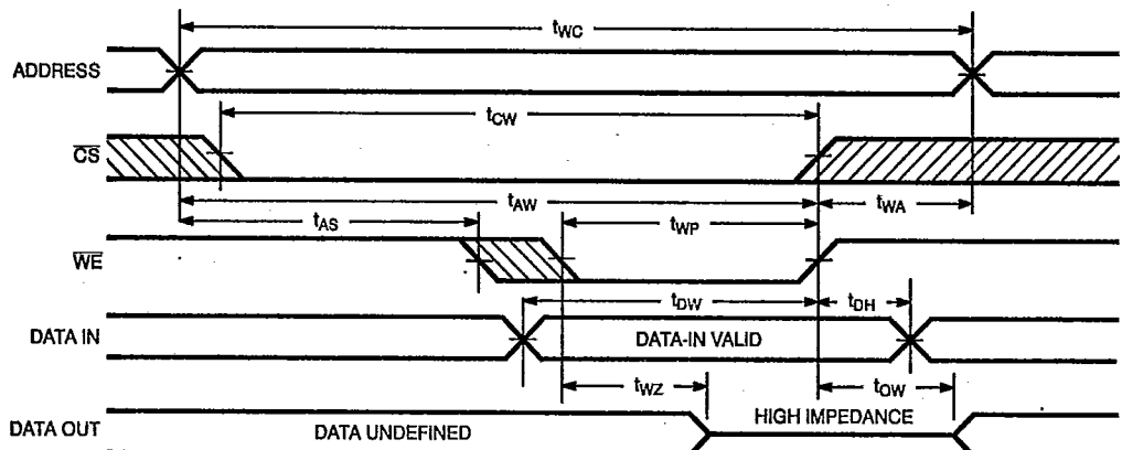
Write Cycle No. 1 ( \overline{WE} Controlled)
